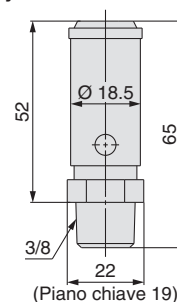
Safety valve: VBAT-R, VBAT-S
