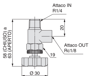
Drain valve: VBAT-V1
